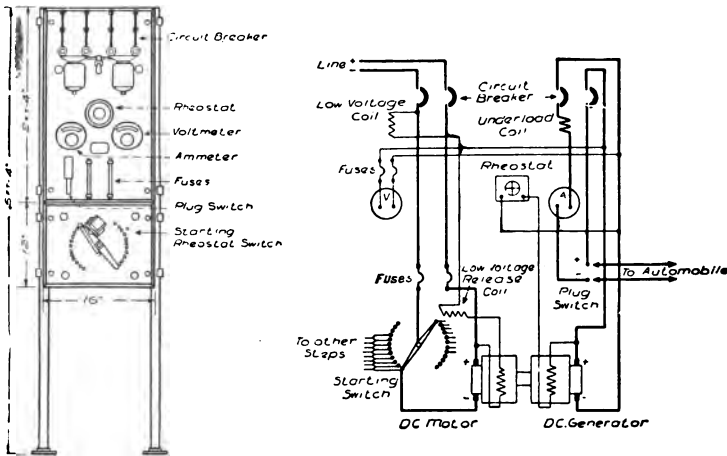
FIGS. 321, 322.—Switchboard and Motor-generator Circuit Connections for Charging a Battery from Direct Current Mains.
